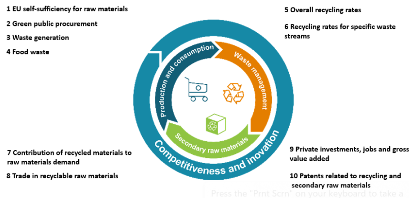
Picture 2. Indicators of CE in EU
