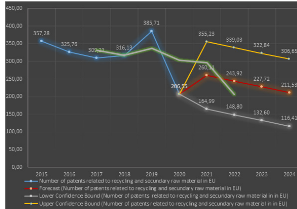
Picture 3. Trend analysis and forecasting for EU countries
